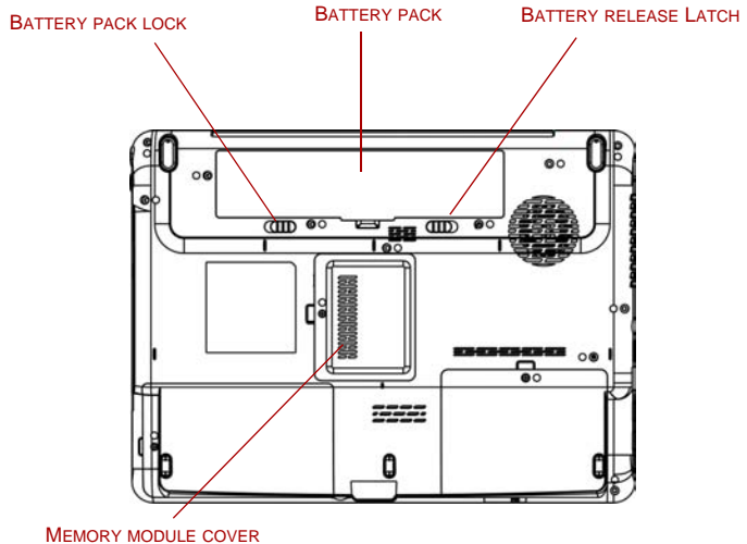
Figure 2-5 The underside of the computer
